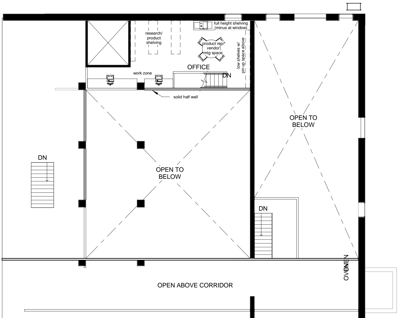
2 Mezzanine Plan - 441 SF 3/32" = 1'-0"
