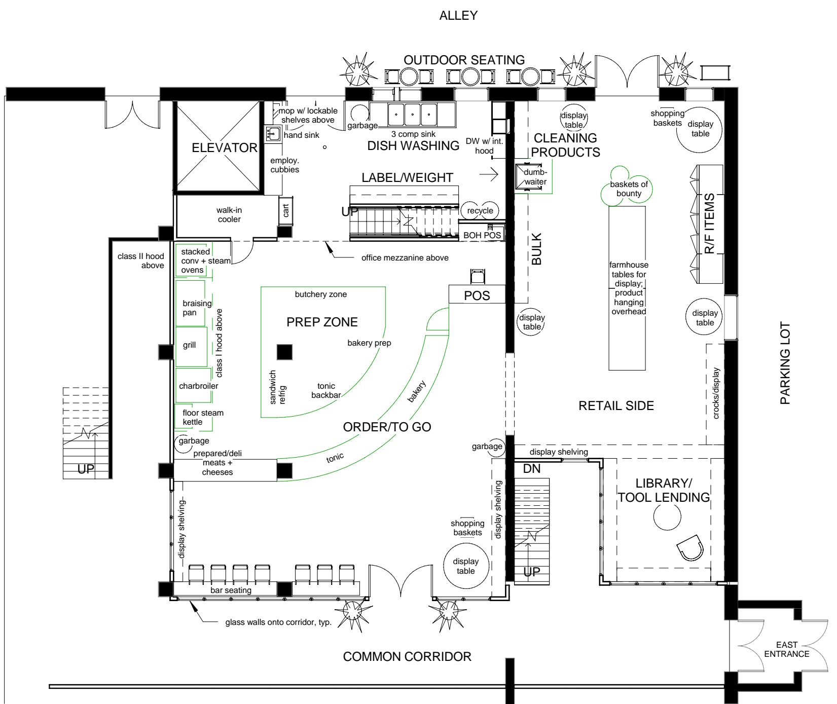
1 First Floor Plan - 2,992 SF 3/32" = 1'-0"
